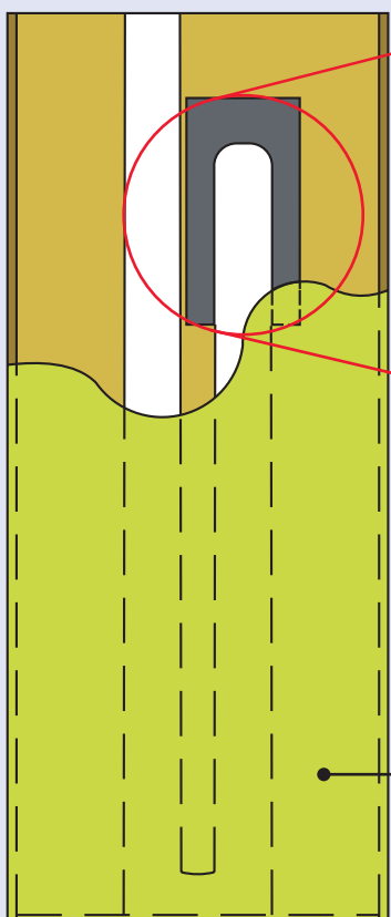
Booster Cross Section with Top-Hat pellet.
